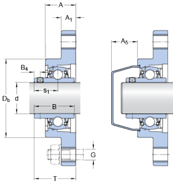
FYTWK 50 LTA Bearing 2D drawings and 3D CAD models
